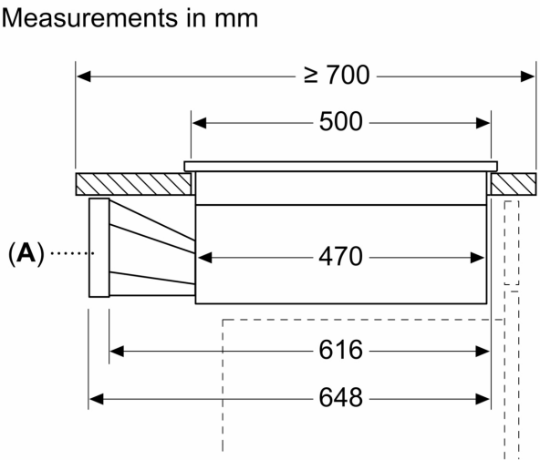
A: Adapter round-flat
